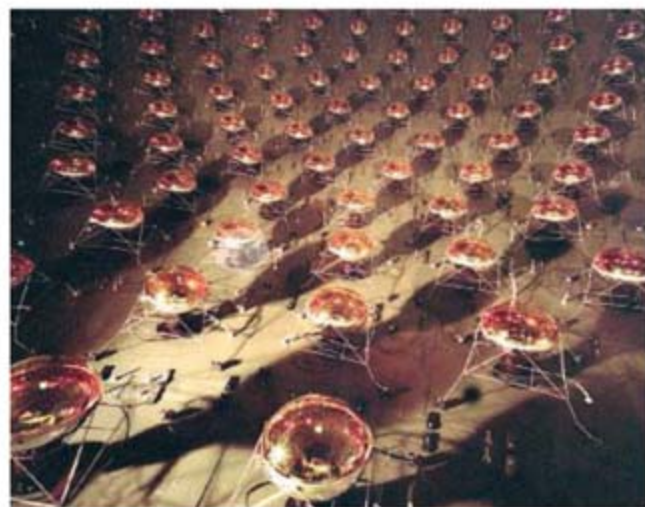
No trace. MiniBooNE's sensor array failed to confirm earlier hints of noninteracting "sterile" neutrinos.
